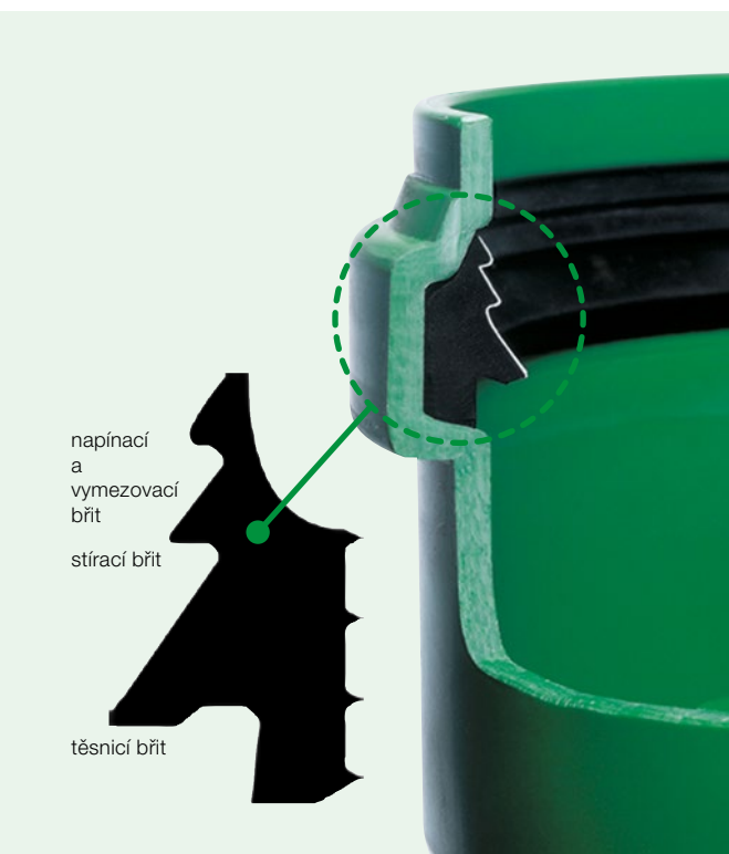
Wavin KG 2000 PP
