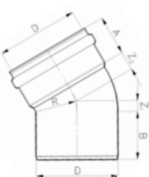
Koleno 30°
